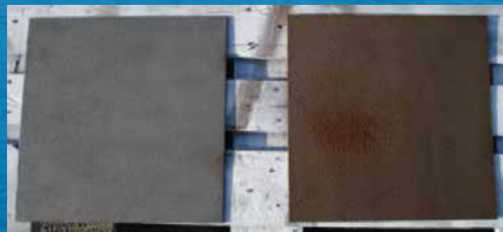
Figure 11. Efficiency testing of corrosion inhibitors in wet blasting process, NCP shipyard, Šibenik
